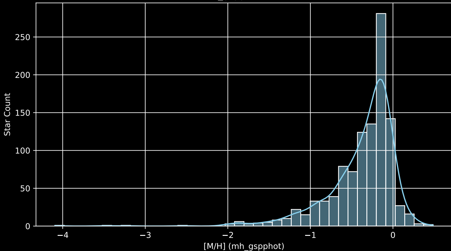
APOGEE DR17 Field: [Omegacen [M/H] (mh_gspphot) (n= 1066)
