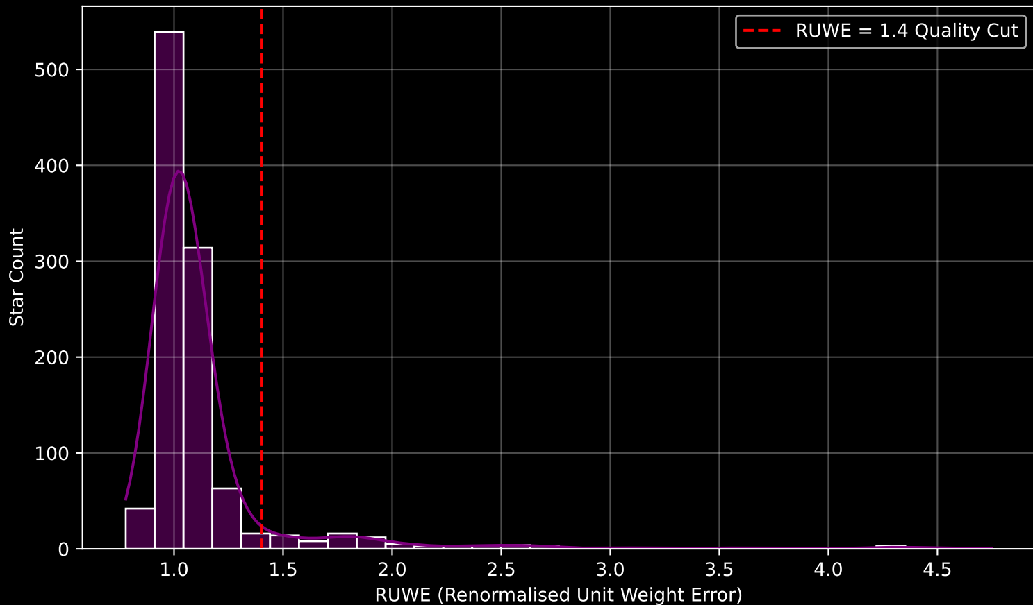
GAPOGEE DR17 Field [Omegacen] RUWE Distribution (n= 1059)
