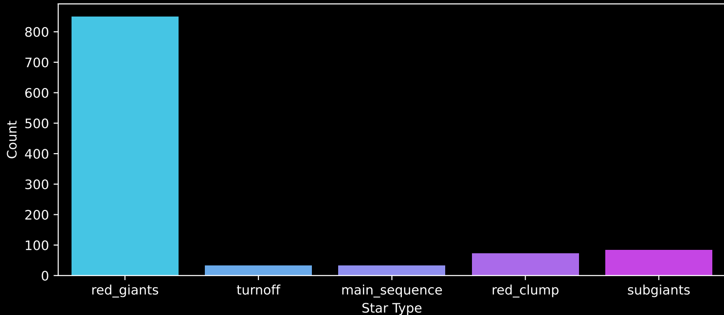
APOGEE DR17 Field: [Omega cen ] Count plot of Star Type
