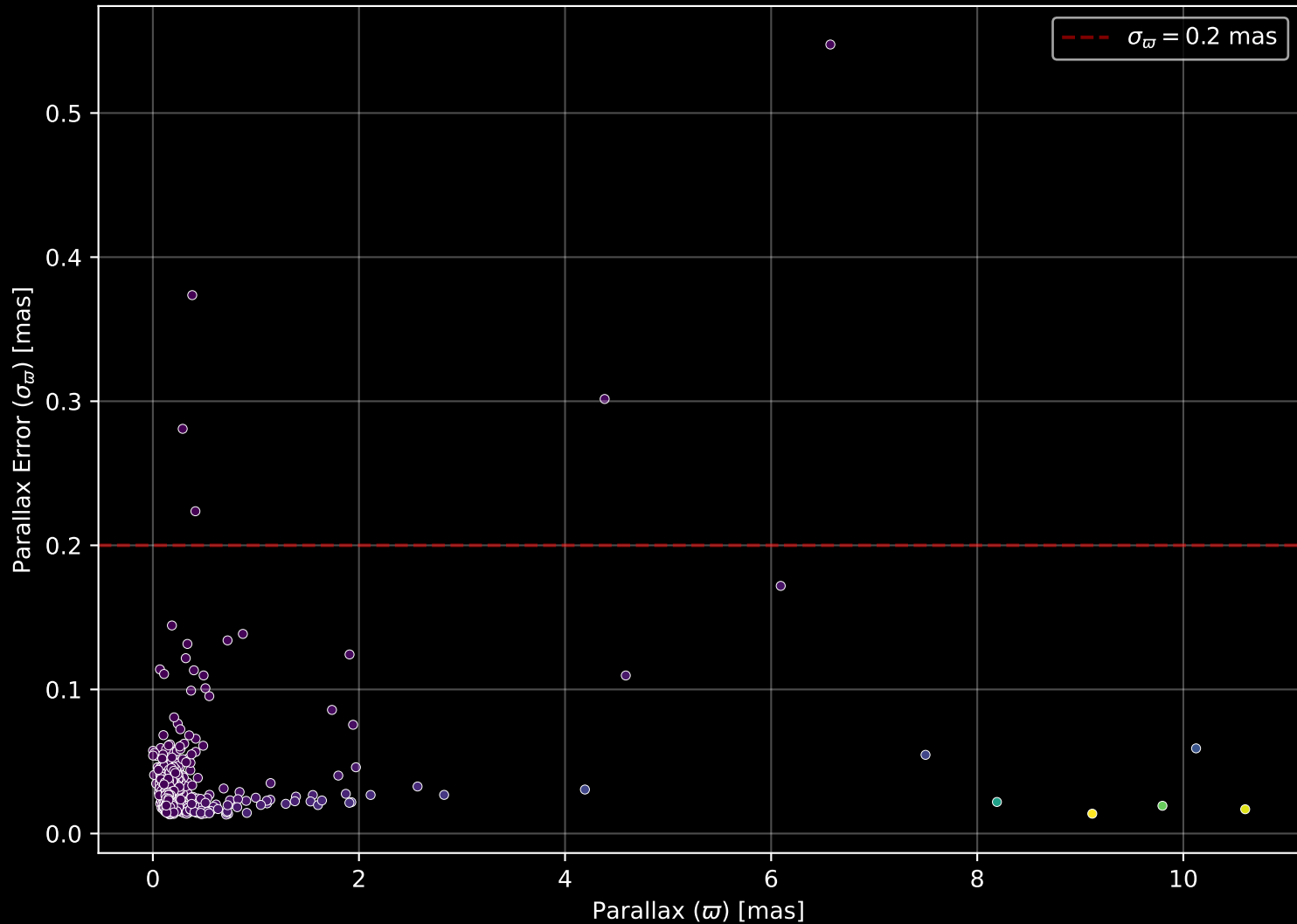
APOGEE DR17 Field: [Omegacen] Parallax Quality (n= 1069)
