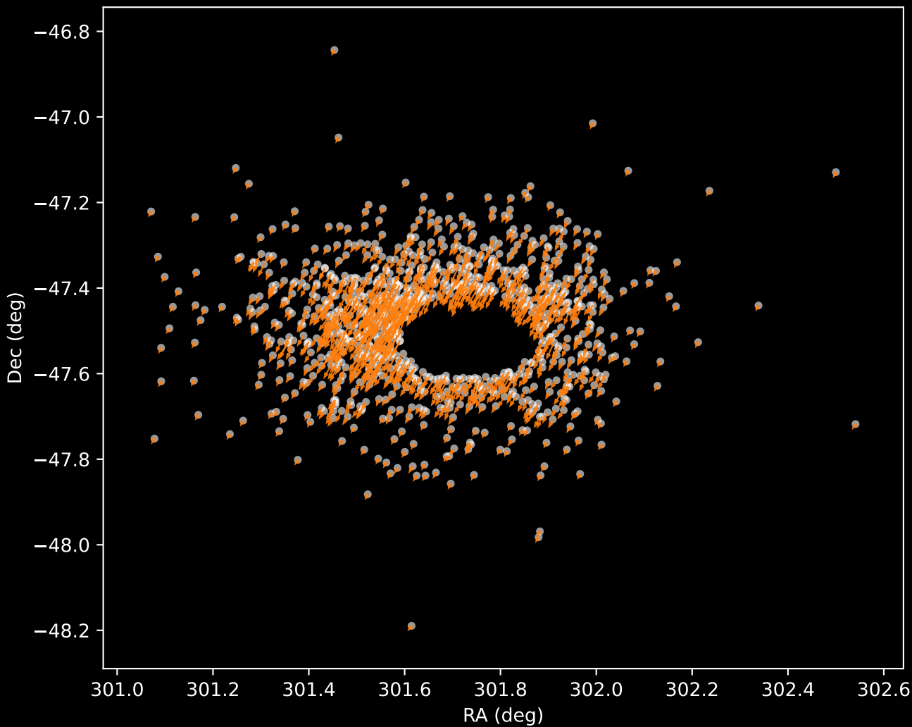
APOGEE DR17 Cluster 2 Proper Motion Vectors (n=947)
