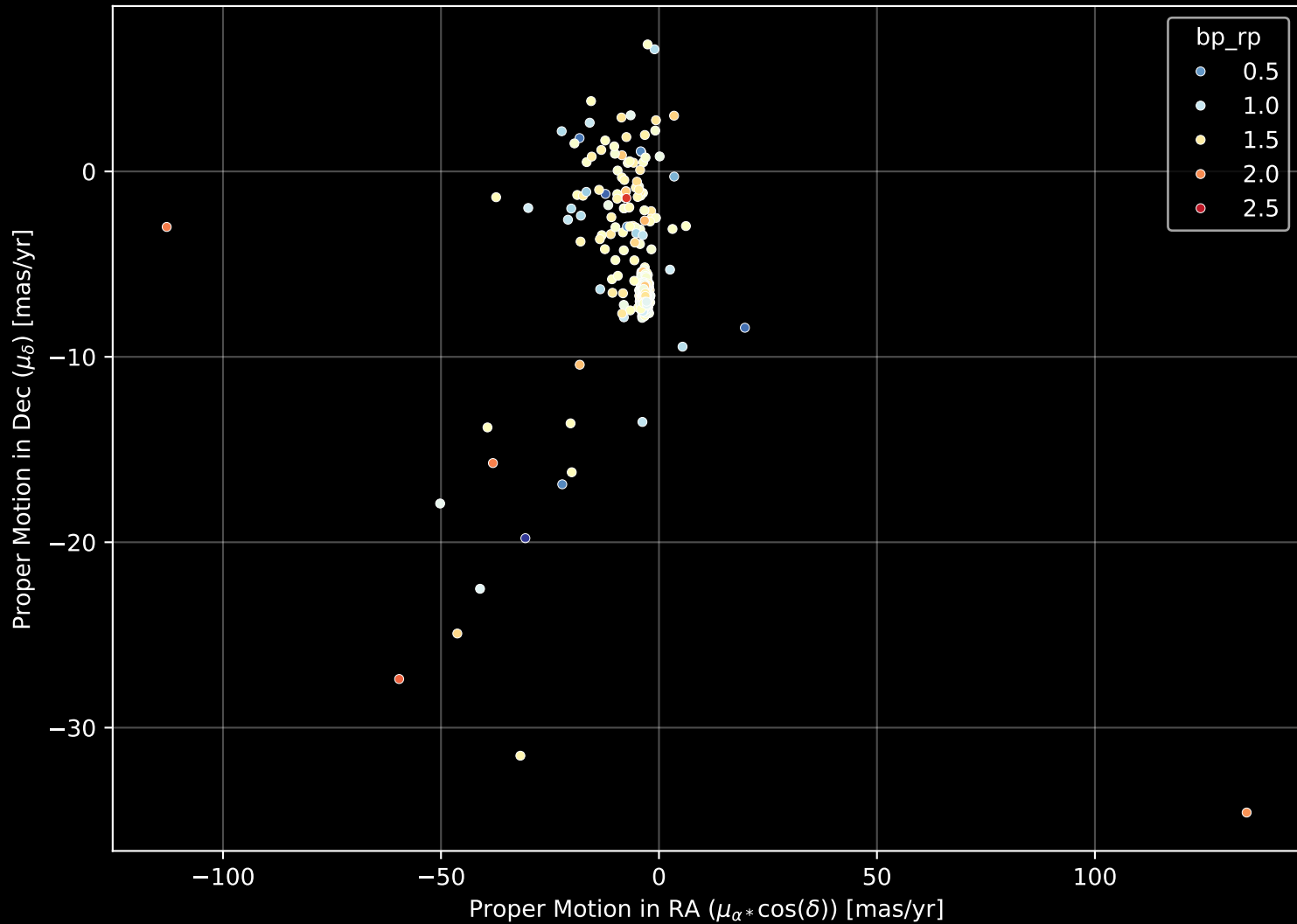
APOGEE DR17 Field: [Omegacen] Proper Motion Diagram (n= 1069)
